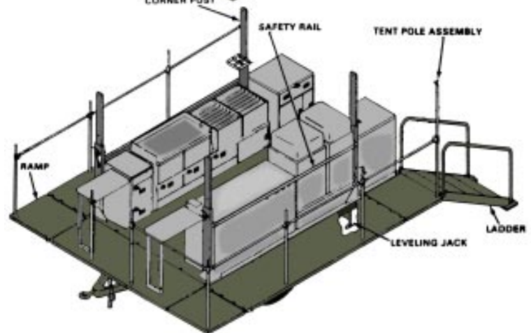
Deployed Foul Weather Tentage Configuration
